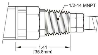
Strain relief with 1/2" Conduit Fitting
