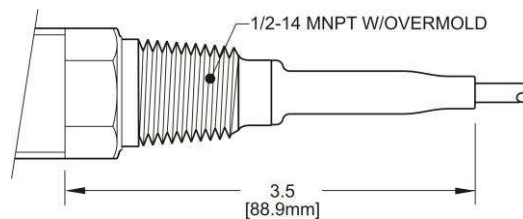
Molded Cable Seal with 1/2" Conduit Fitting
